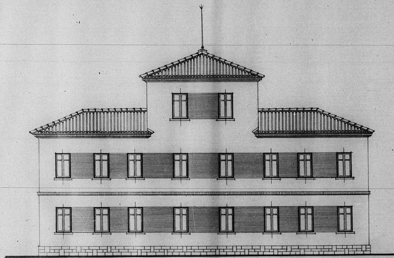
Alzado principal
