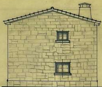
LATERAL
