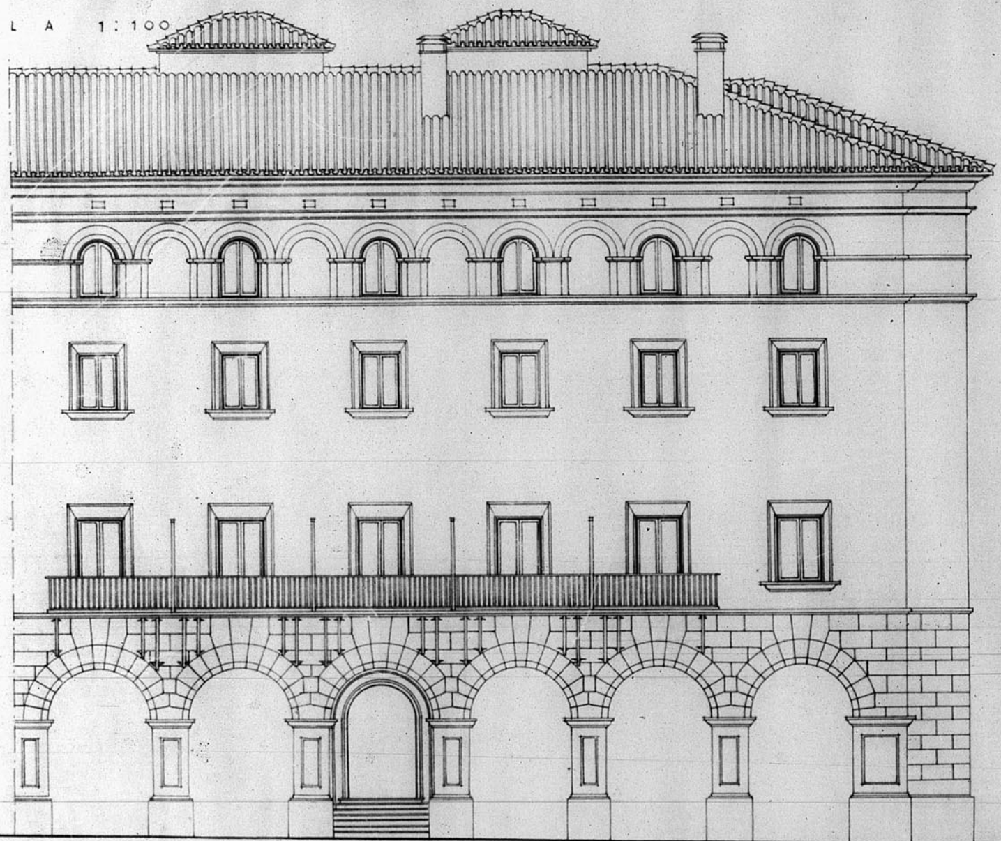
ALZADO PRINCIPAL
